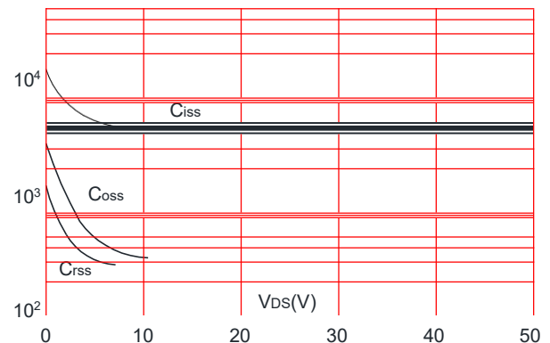
Figure 6: Capacitance Characteristics
